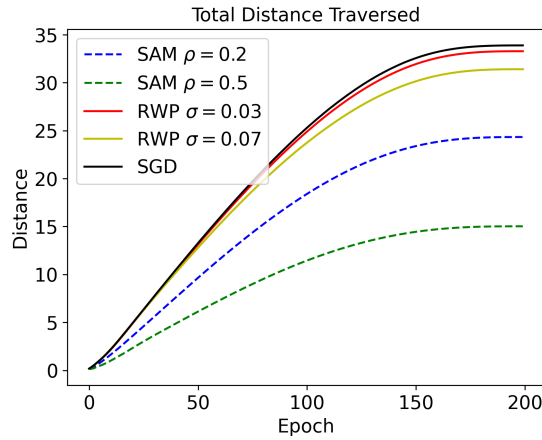
Figure 9. (a) Plot of the ResNet-18 update gradient norm \|\nabla L\|_2 as a function of training epoch for SGD, SAM, and RWP on Cifar-100. (b) Plot of the total distance traversed during training, \sum_{i=1}^N \|w_{t+1} - w_t\|
