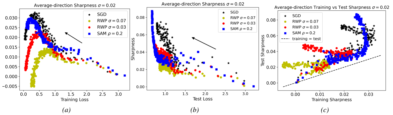
Figure 10. (a) Plot of ResNet-18 Cifar-100 average-direction sharpness for \sigma = 0.02 . as a function of training loss. (b) Plot of average-direction sharpness as a function of test loss for \sigma = 0.02 . (c) Plot of test sharpness as a function of training sharpness for \sigma = 0.02 .
